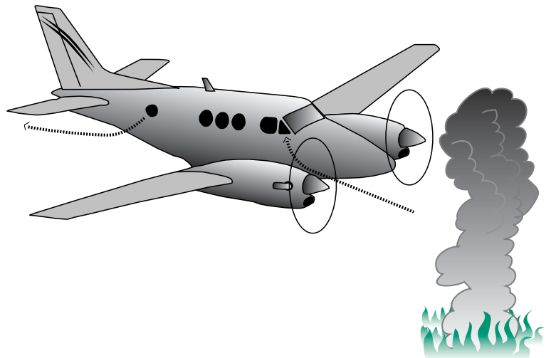
Figure 4. Example of the duct system showing how forest fire smoke was moved through the spectrometer as the airplane flew through forest fire smoke.
